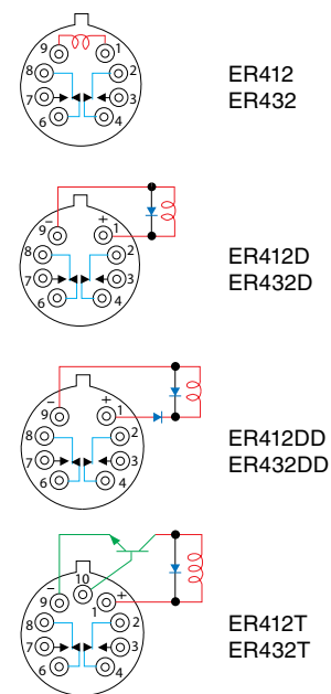
Schematics as viewed from terminals
