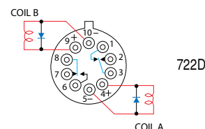
SCHEMATIC (Coil A Last Energized) (Bottom View)
