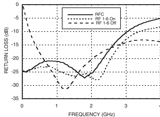
Return Loss [1]
