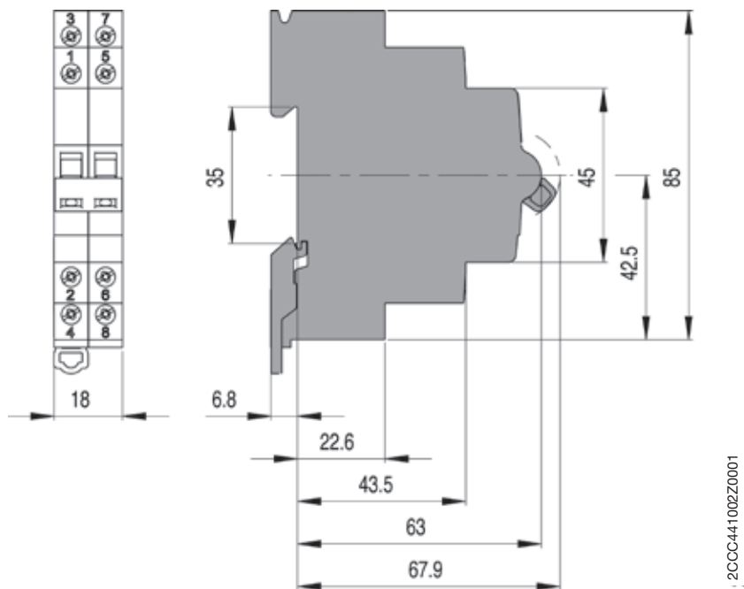
Switch, 3+4-pole
