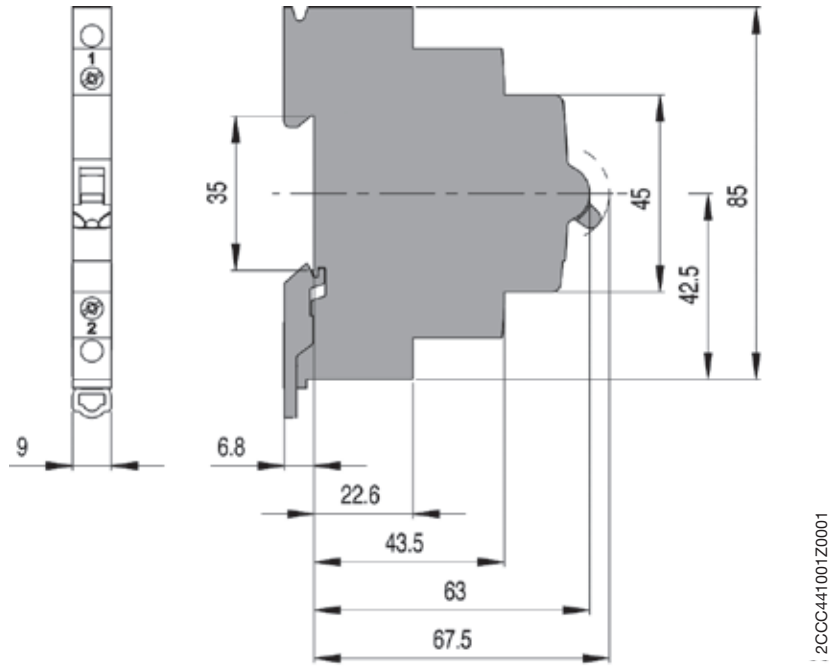
Switch, 1+2-pole
