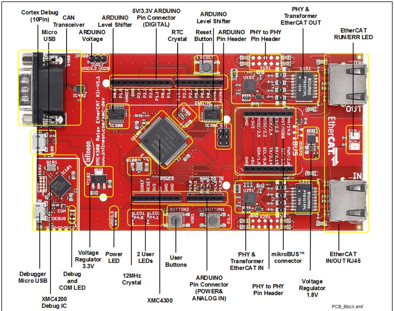
Figure 2 PCB of the XMC4300 Relax EtherCAT® kits
