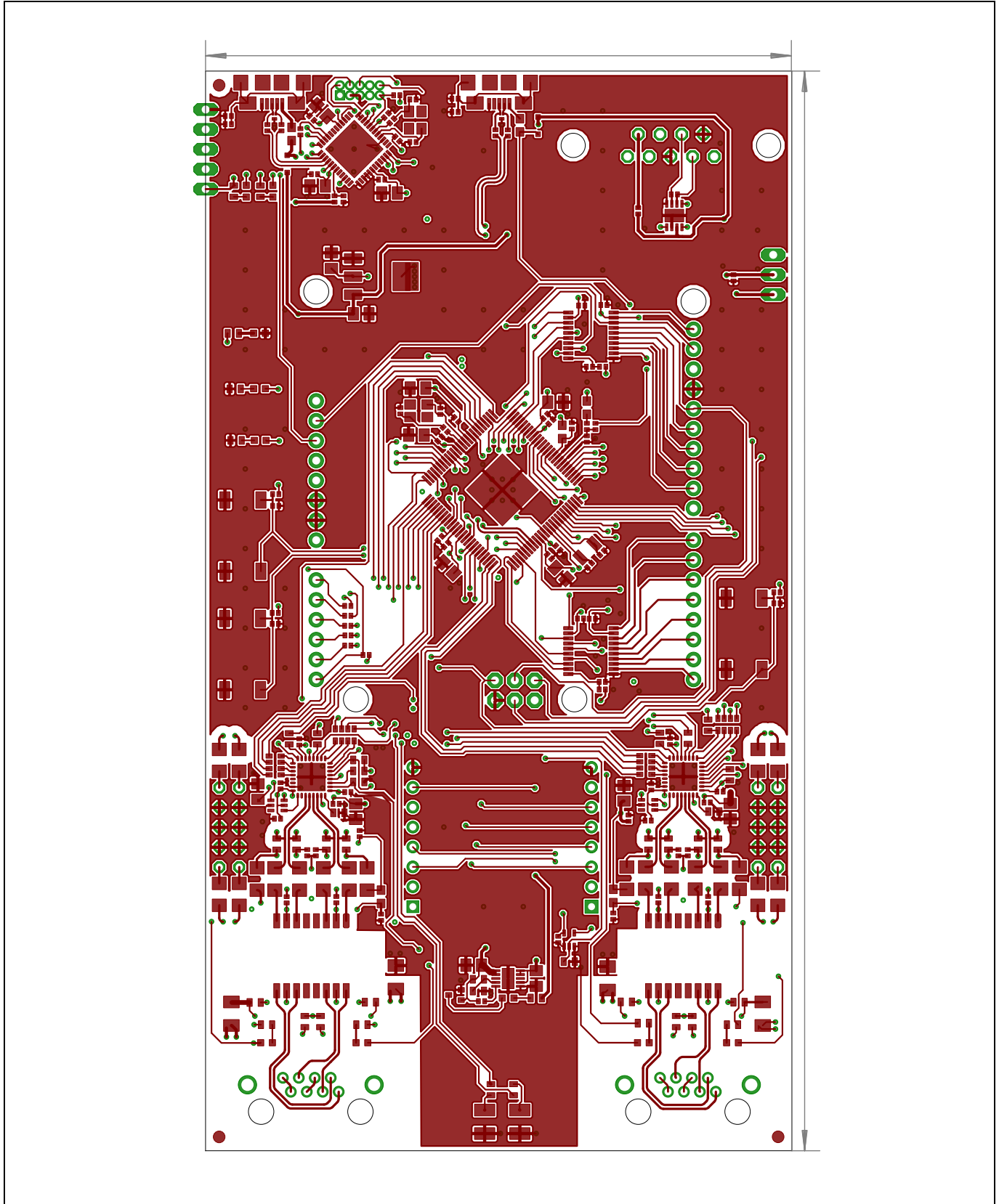
Figure 11 Components placement and geometry
