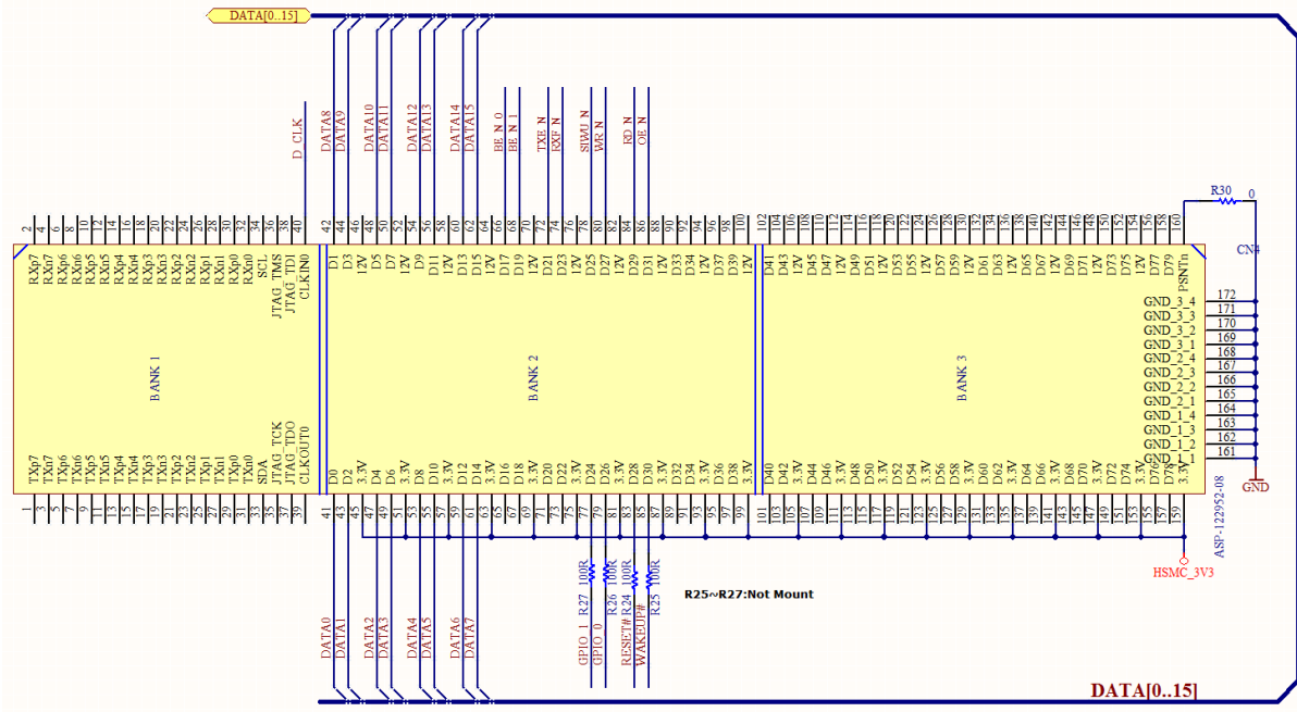
Figure 3-4 Schematics: HSMC_UMFT600A
