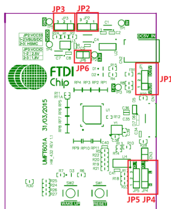
Figure 4-1 Jumpers Locations
