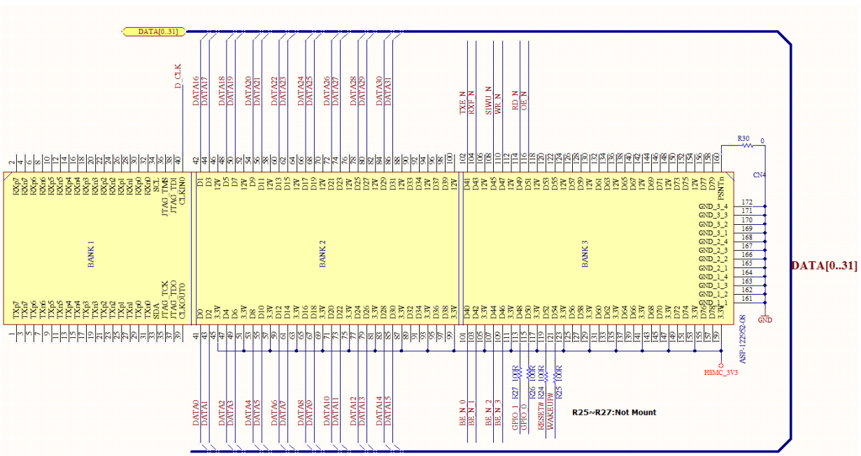
Figure 3-5 Schematics: HSMC_UMFT601A
