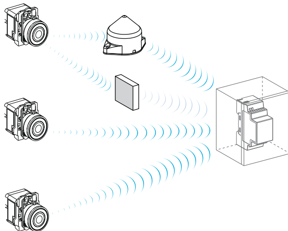
Figure B: Transmission between 3 Transmitters and 1 Receiver
