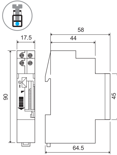
12.11 Screw terminal
