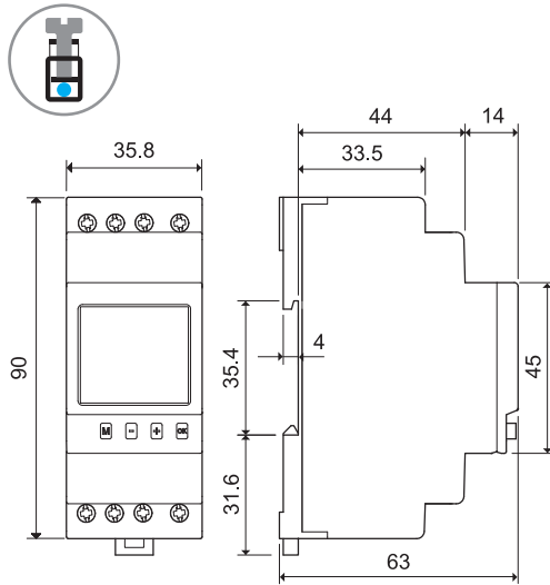
12.51/12.81 Screw terminal
