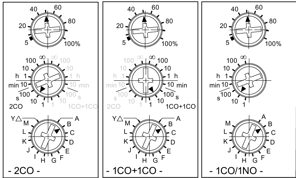
2CO 1CO+1CO 1CO - 1 CO contact 2 CO contacts in parallel, delayed contacts 2 CO contacts, 1x delayed contact 1x instantaneous contact 1NO - 1 semiconductor
