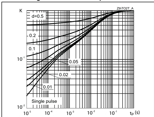
Figure 10. Thermal impedance
