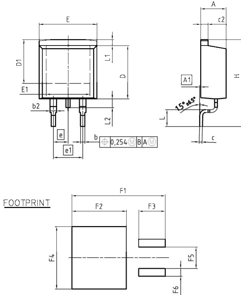
PG-TO263-3
