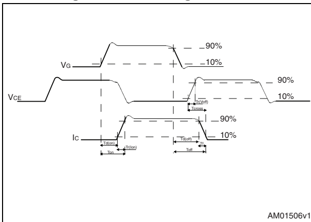
Figure 30. Switching waveform
