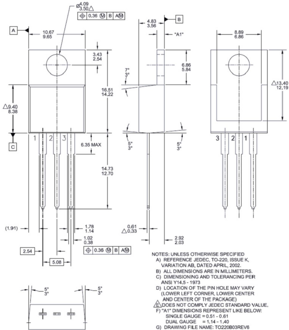
Figure 24. TO-220 3L - TO-220, MOLDED, 3LEAD, JEDEC VARIATION AB
