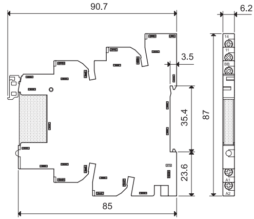
39.40 39.41 Screw terminal
