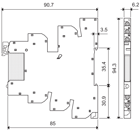
39.80 39.81 Screw terminal
