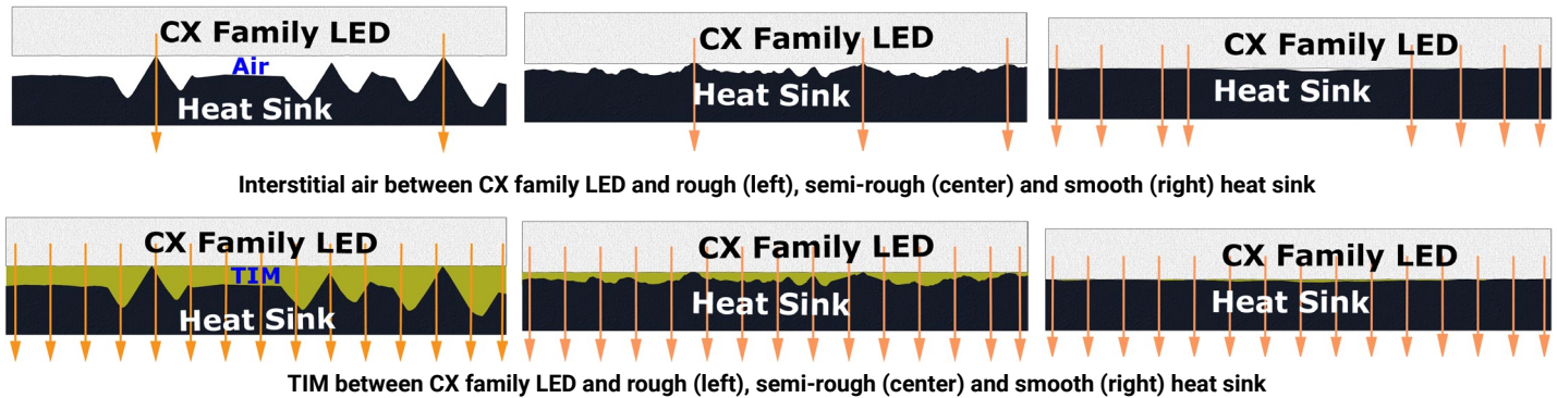
Figure 13: TIM fills the voids between CX family LED and heat sink
