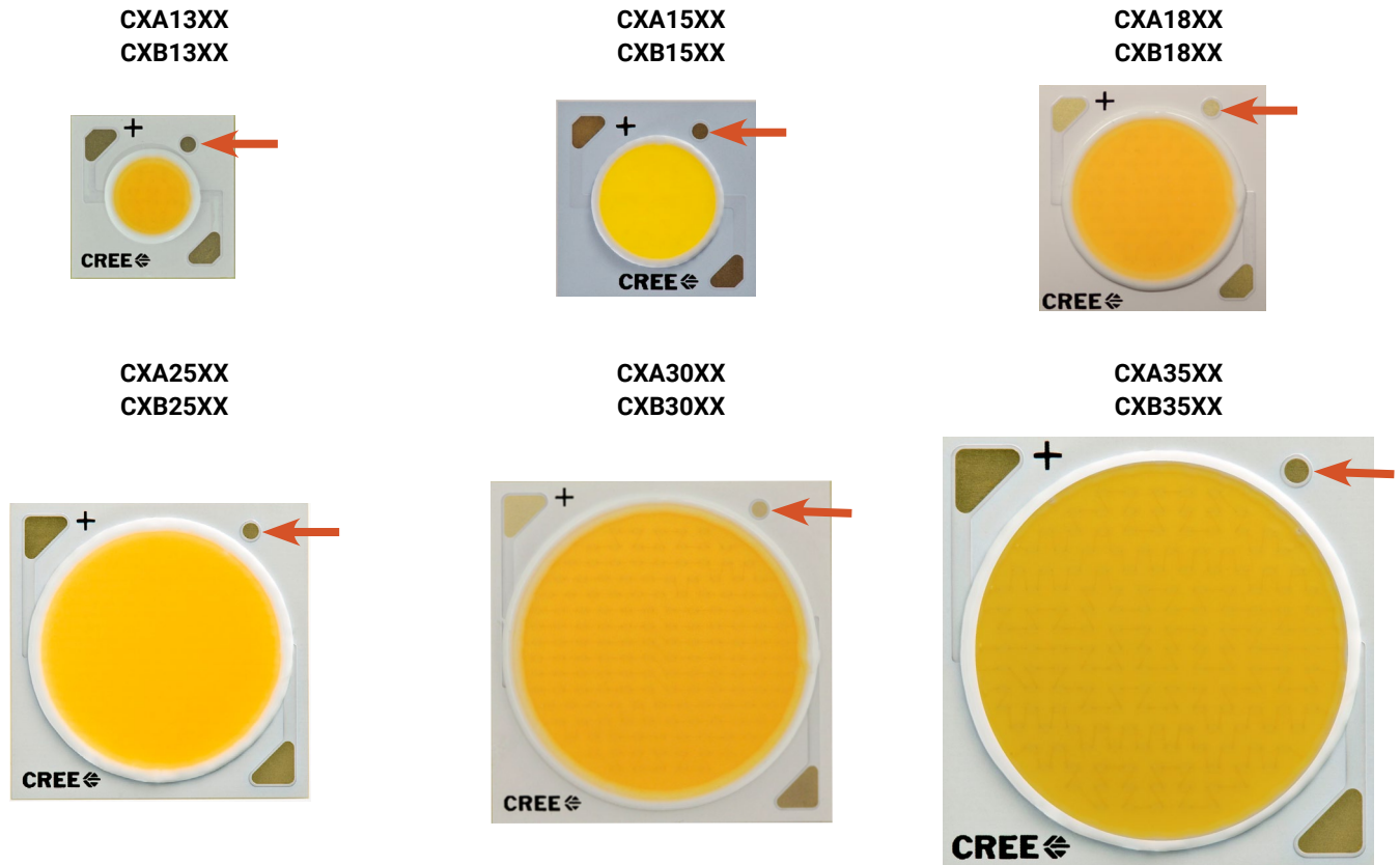
Figure 8: Tc measurement point for CX family LEDs
