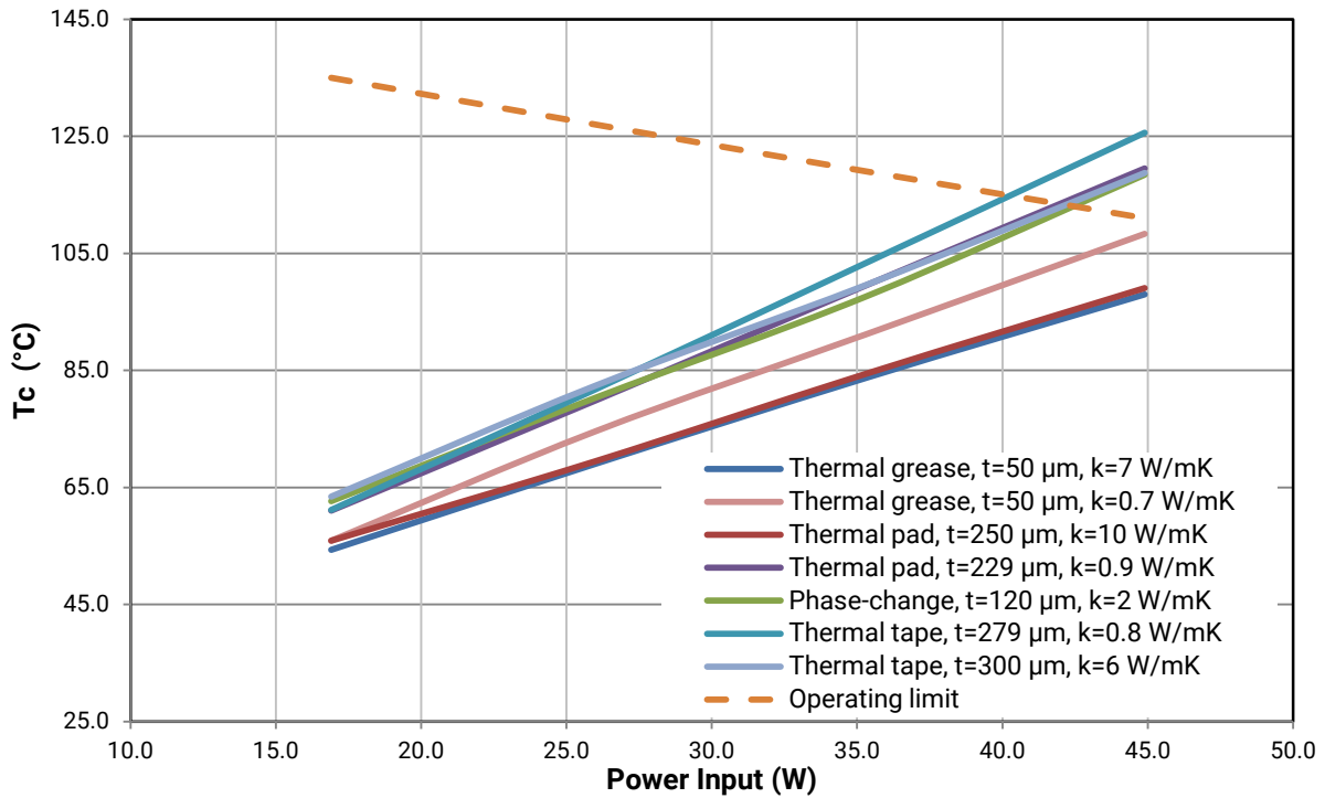
Figure 14: CXA2540 Tc vs. power
