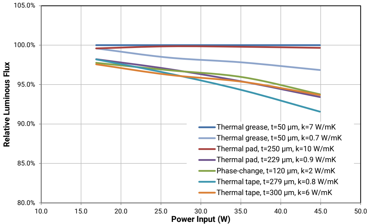
Figure 15: CXA2540 relative luminous flux vs. power
