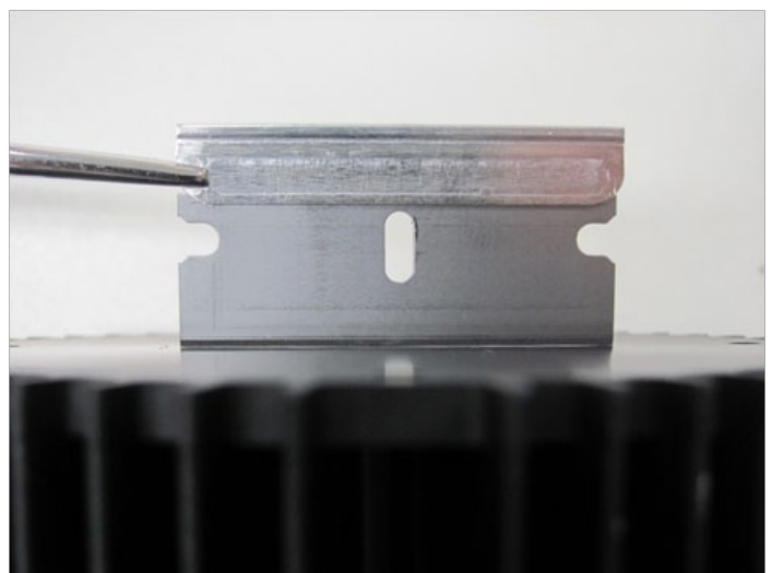
Figure 12: Checking heat sink flatness, left: a gap below the razorblade edge, right: no gap below the razorblade edge
