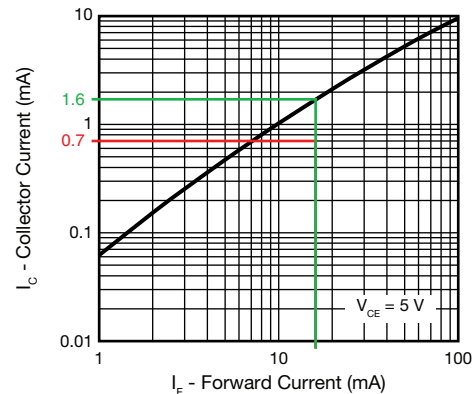
Fig. 2 - Collector Current vs. Forward Current
