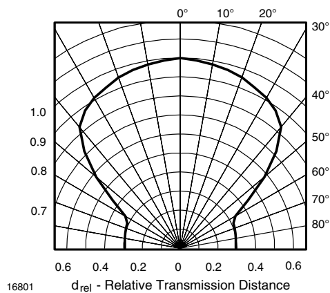
Fig. 12 - Directivity
