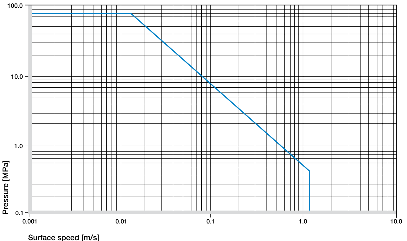
Graph 01: Permissible pv values for iglidur® G with a wall thickness of 1 mm dry running against a steel shaft at +20 °C, mounted in a steel housing
