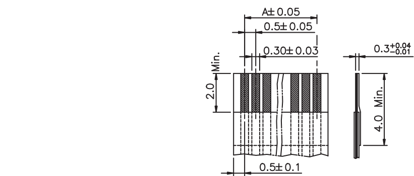
ACCOMODATED FFC/FPC
