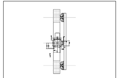
GDL Coupled with structural aluminum extrusion material and OSP-E actuator
