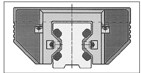
Full profile snap-on wiper
