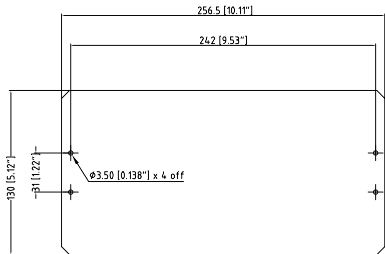
Anodised Front Panel 2mm Thick
