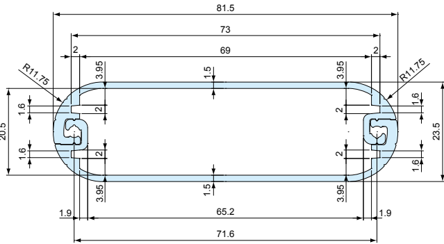
MX / MXA 2-10-□
