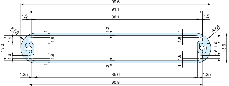
MX / MXA 2-10-□
