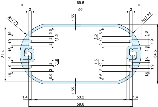
MX / MXA 4-7-□
