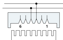
Rear View of Terminal Connection Block
