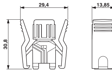
Dimensioned drawing
