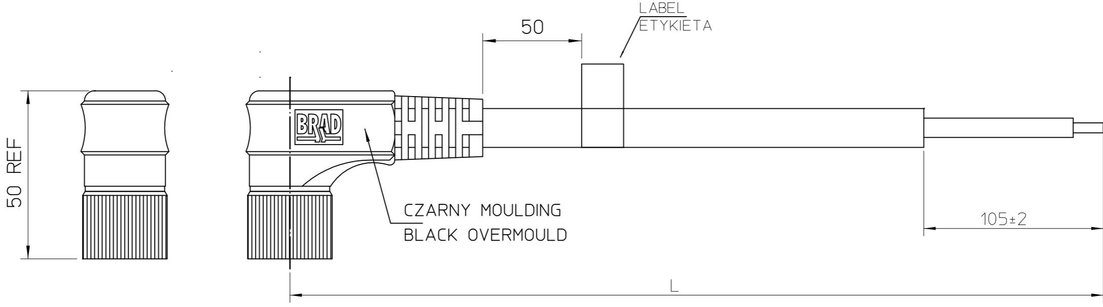
WIDOK OD STRONY DRUTOW VIEW FROM WIRES SIDE
