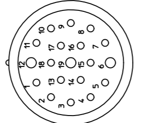
WIDOK OD STRONY CZOLA VIEW FROM FRONT SIDE
