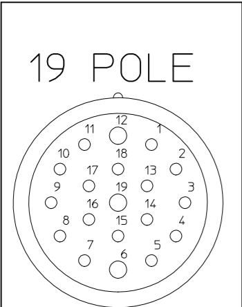
WIDOK OD STRONY DRUTOW VIEW FROM WIRES SIDE
