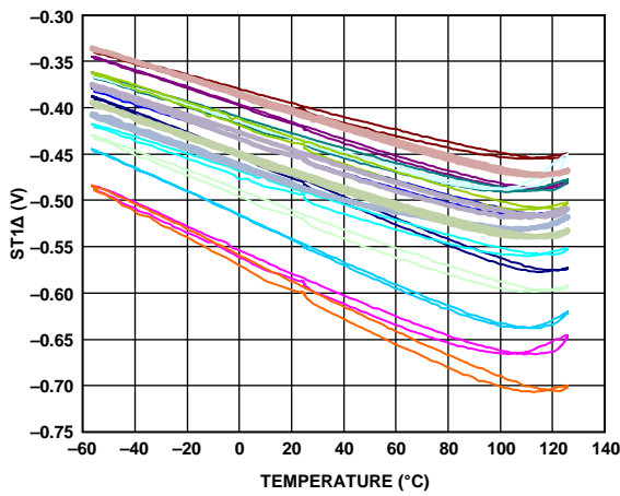
Figure 11. ST1 Output Change vs. Temperature, 16 Parts in Sockets
