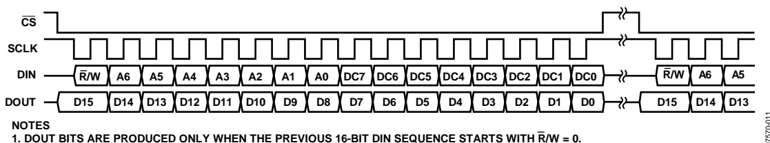
Figure 11. SPI Communication Bit Sequence
