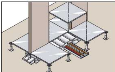
PFC Corofil Intumescent Pillows forming cavity barrier under raised access floor.
