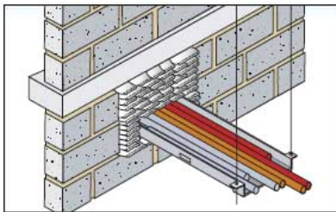
PFC Corofil Intumescent Pillows friction fitted between services and firewall.
