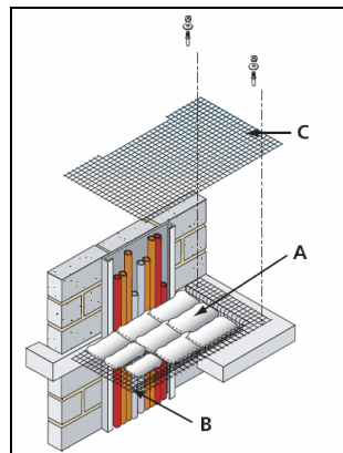
PFC Corofil Intumescent Pillows supported by mesh cage in service riser floor.
