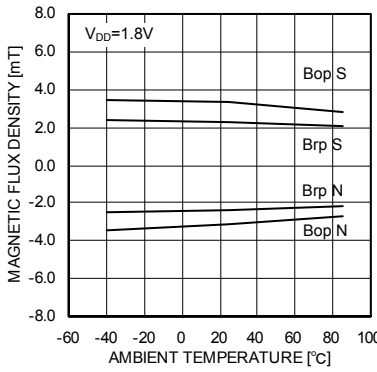
Fig.36 Bop, Brp– Ambient temperature
