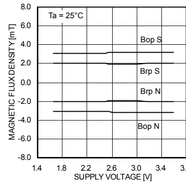
Fig.37 Bop, Brp– Supply voltage
