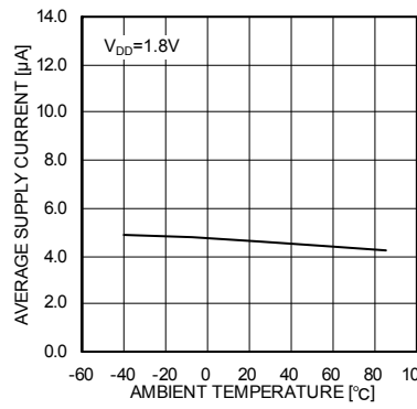
Fig.40 I DD – Ambient temperature
