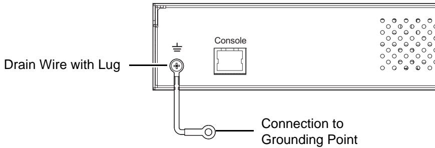
Figure 18: Grounding Connection
