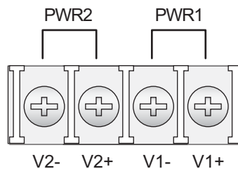
Figure 20: Terminal Receptor: Power Input Contacts
