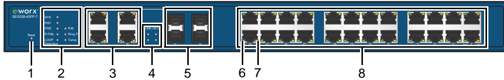
Figure 1: Front View
