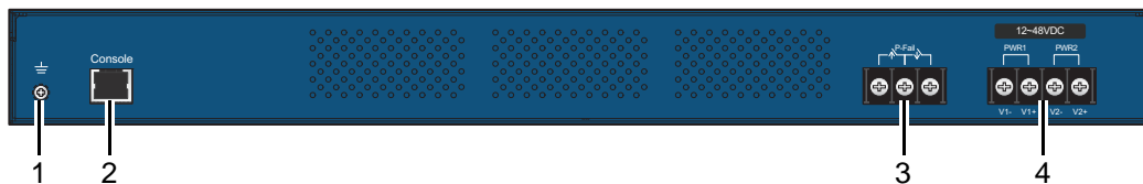
Figure 3: Rear View
