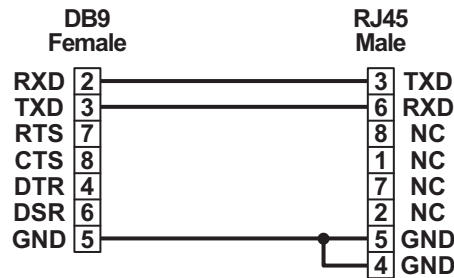
Figure 16: Pin Assignment
