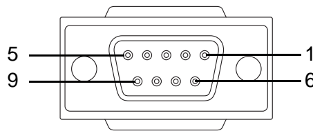
Figure 15: DB 9 Pin Position
