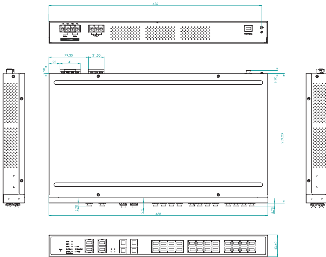
Figure 4: SEGP528T Dimensions
