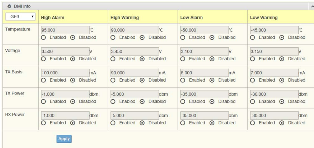
Figure 132: Diagnostics > DDM
