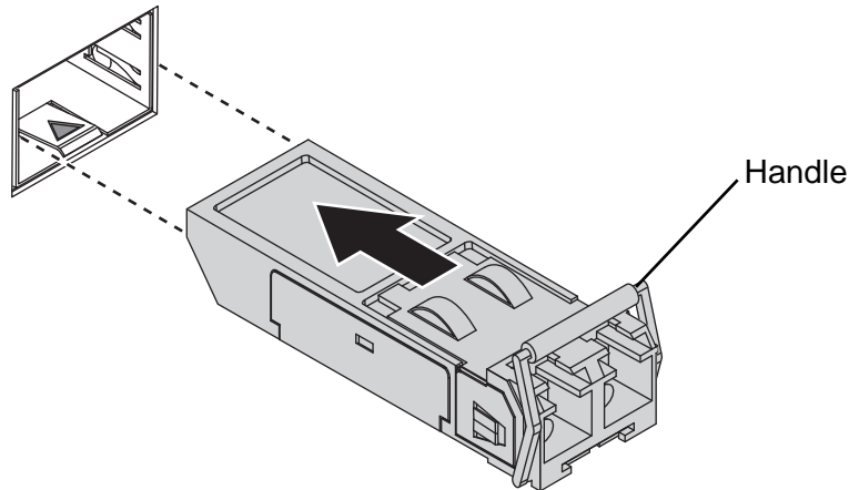
Figure 9: Installing an SFP Transceiver
