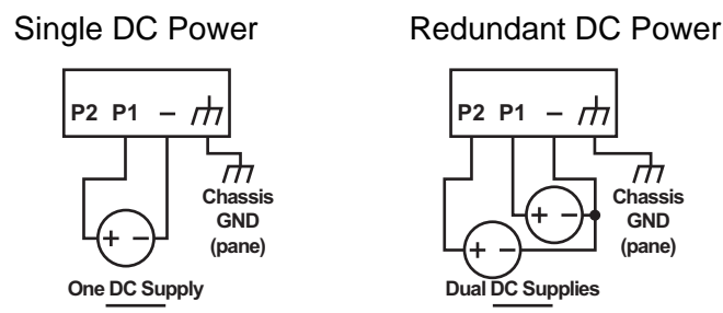
Figure 17: Power Wiring for SE528 Series
