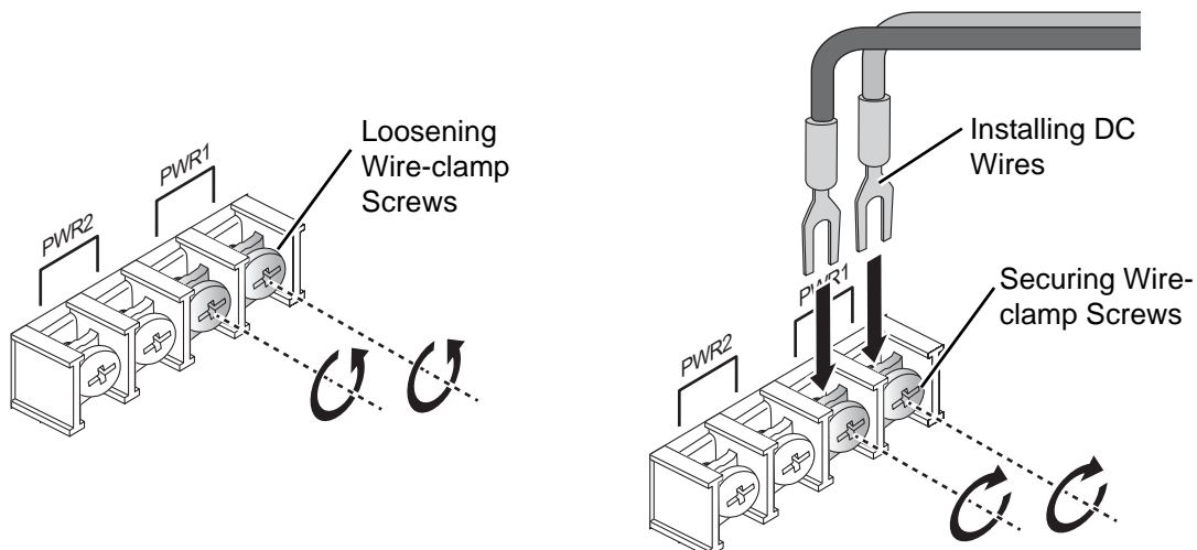
Figure 21: Installing DC Wires in a Terminal Block
