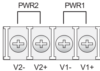
Figure 19: Terminal Receptor: Power Input Contacts
