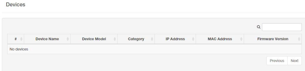
Figure 133: Tools > IXM
