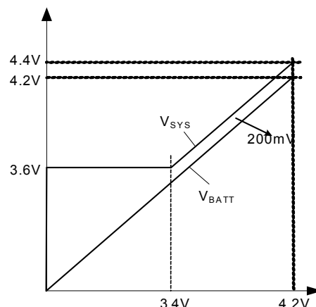
Figure 2 — MP 2617B SYS Regulation Output
