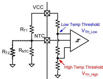
Figure 9—NTC Function Block
