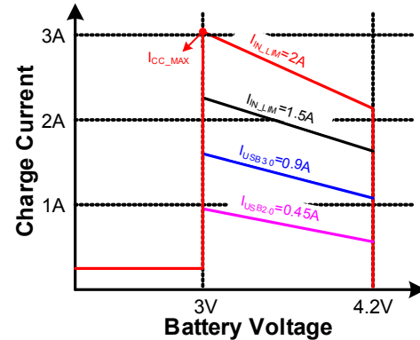
Figure 8— I CHG Variation with Different Input Current Limit
