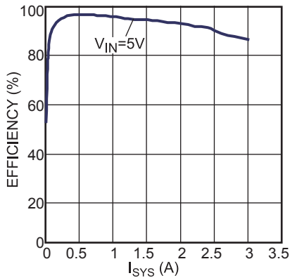
Efficiency vs. System Current
