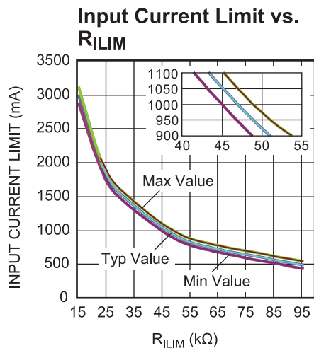
Figure 3 — Input Current Limit vs. R ILIM
