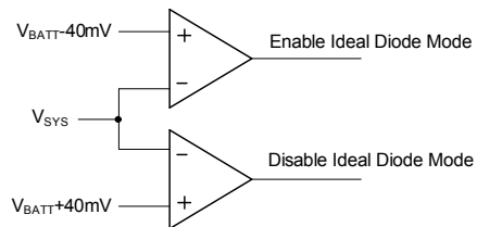
Figure 5—Ideal Diode Mode Enable/Disable
