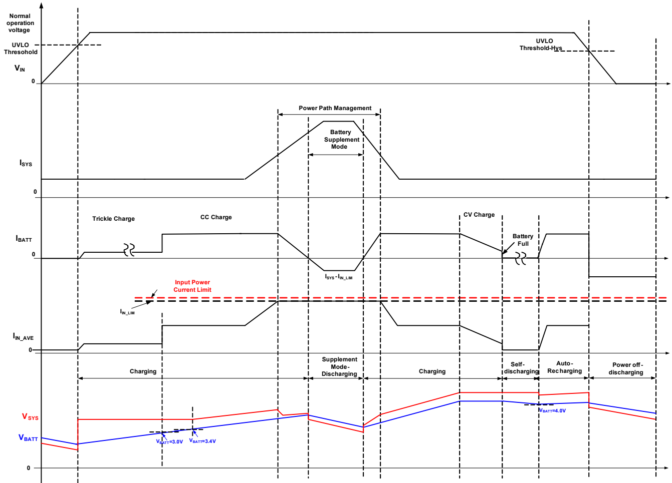
Figure 7— MP2617B Operation Process under No Fault Condition
