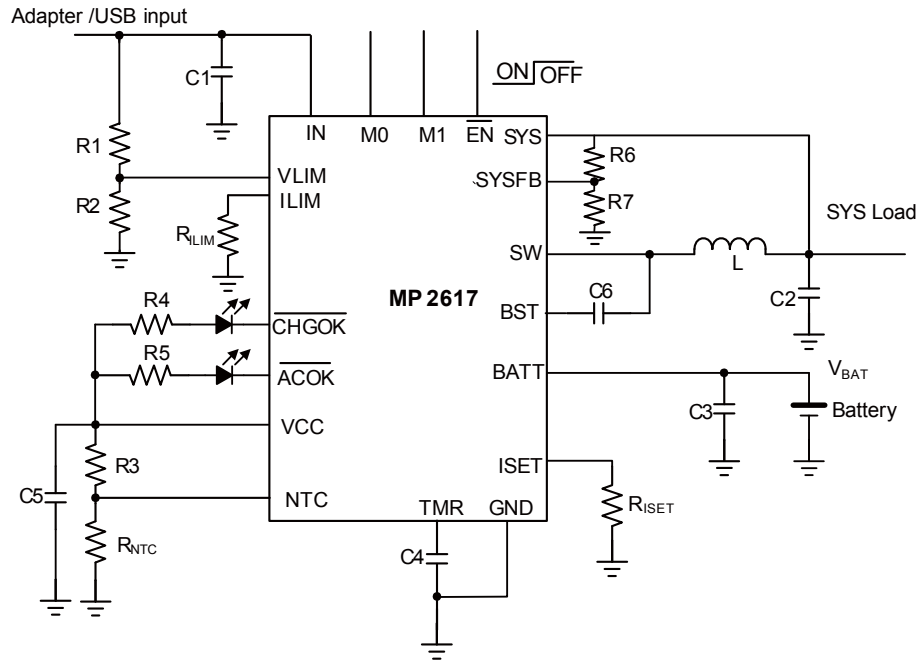
Figure 10—Typical Charge Application Circuit with V_{SYS} Programmed by SYSFB Pin
