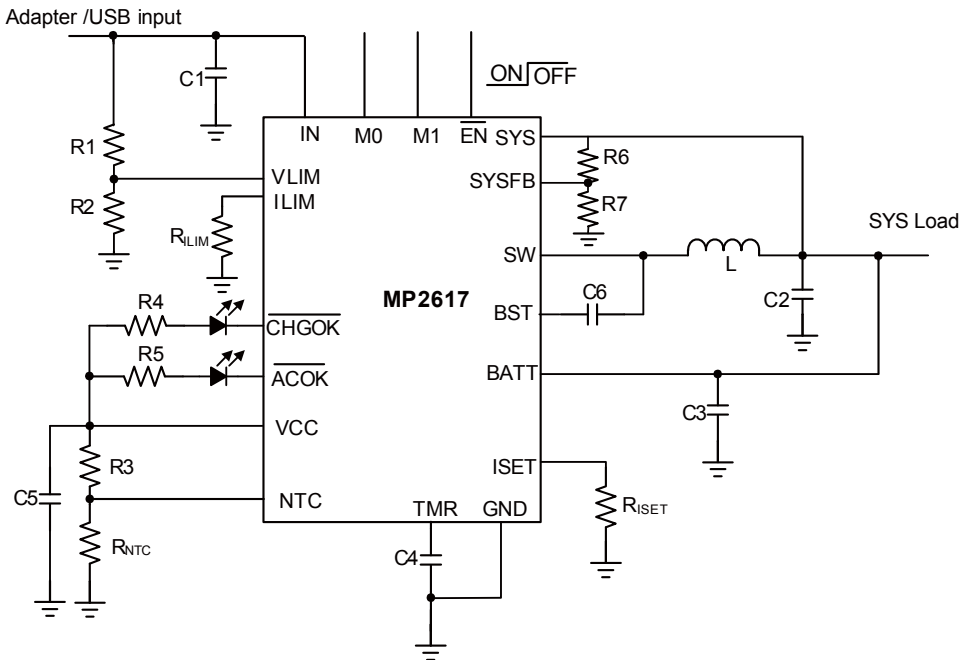
Figure 11—Application with Charger Disabled under No Battery Condition
