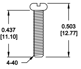
HOUSING SCREW
