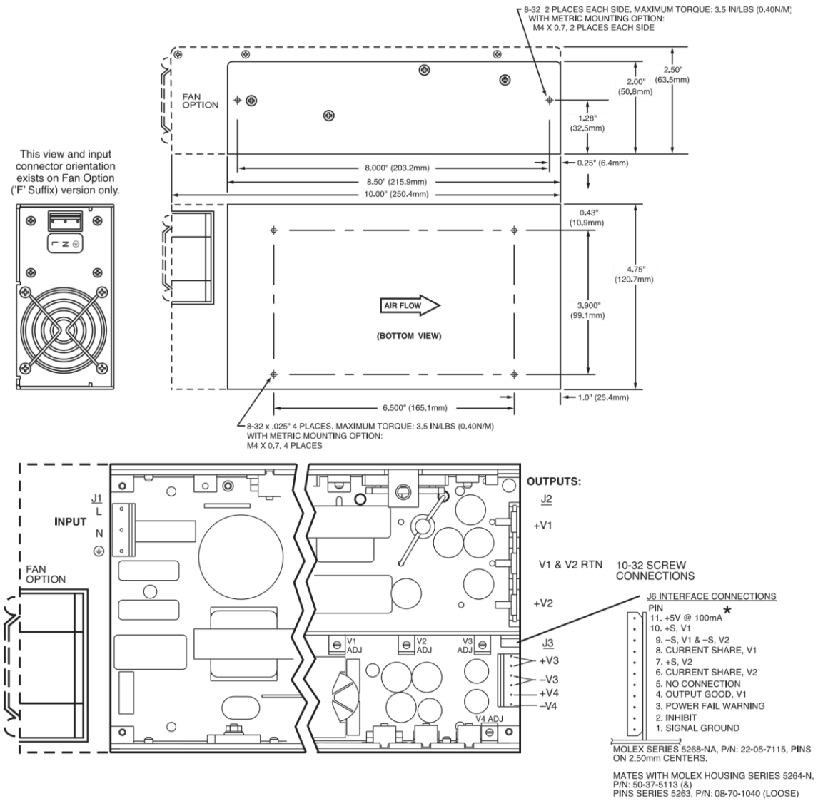
Figure 1. Mechanical Drawing PFC250
