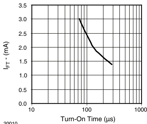
Fig. 8 - I_{FT} (mA) vs. Turn-On Time (µs)
