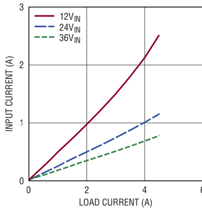
Input vs Load Current V_{OUT} = -5\text{V} , BIAS Tied to LTM8003 GND
