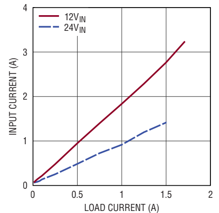
Input vs Load Current V_{OUT} = -18\text{V} , BIAS Tied to LTM8003 GND
