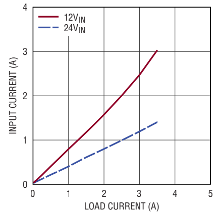
Input vs Load Current V_{OUT} = -8\text{V} , BIAS Tied to LTM8003 GND
