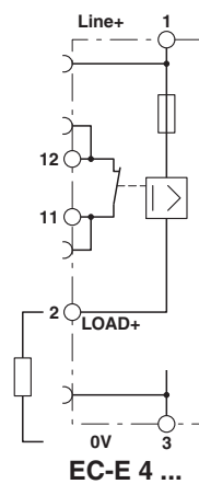
Circuit diagram
